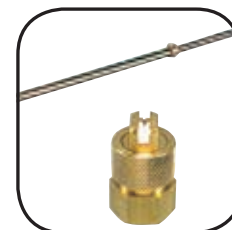
Spray pipe, flat-spray nozzle and quick-action stop valve made from brass: Robust and durable.
